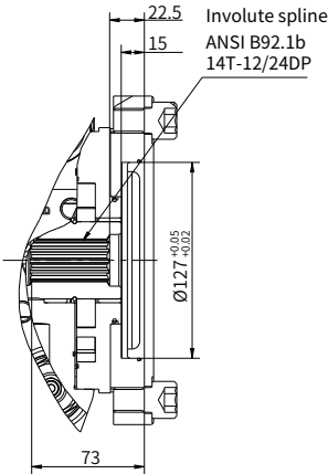
“CC” type through drive
