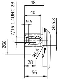
"B4" type spline shaft ANSI B92.1b 1 1/4 in 14T 12/24DP
