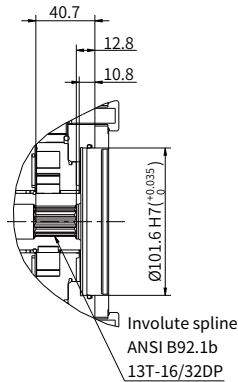
"B1" type through drive
