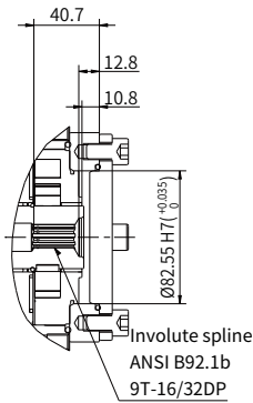
"A1" type through drive
