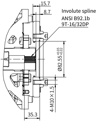
“A1” type through drive
