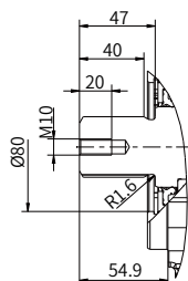
“C8” type spline shaft
