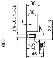
"B3" type spline shaft ANSI B92.1b 1 in 15T 16/32DP
