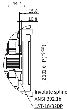
"B3" type through drive
