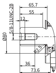
“C9” type spline shaft
