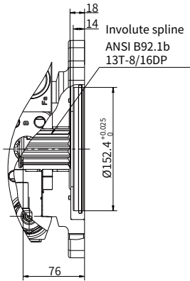
“D1” type through drive
