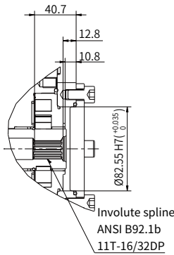
"A2" type through drive
